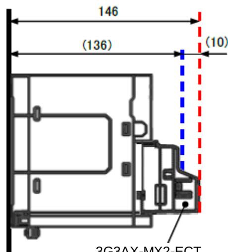
3G3AX-MX2-ECT
